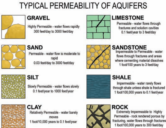
Figure 6. Permeability ranges for aquifer materials.
